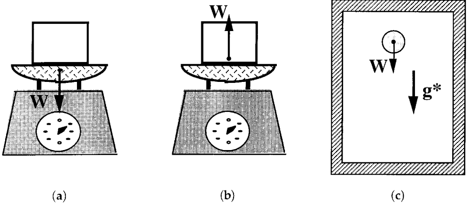
Figure 1. Operational definitions of weight: (a) weight is the force exerted on the support by the object; (b) weight is the force exerted on the object by the support; and (c) weight is the force exerted on the object causing its spontaneous fall with acceleration g^* , as measured in the laboratory.
